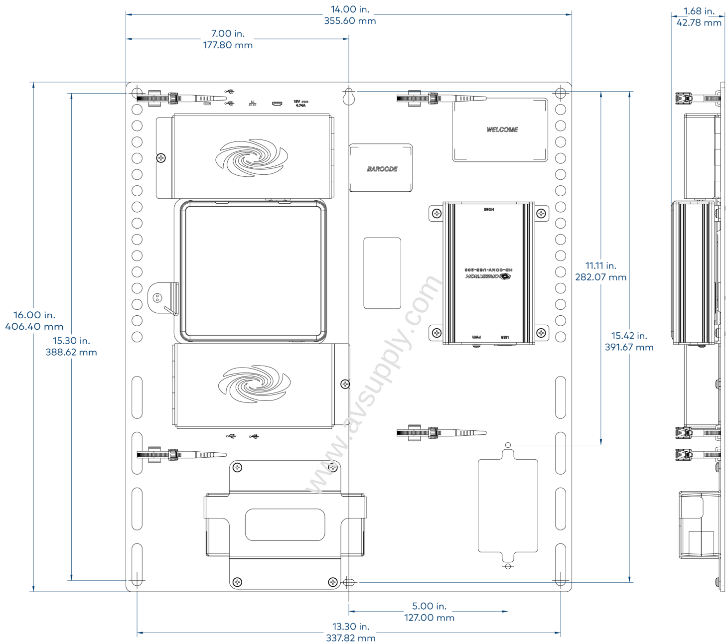
UC-BRKT-100-SD-Z-ASSY
